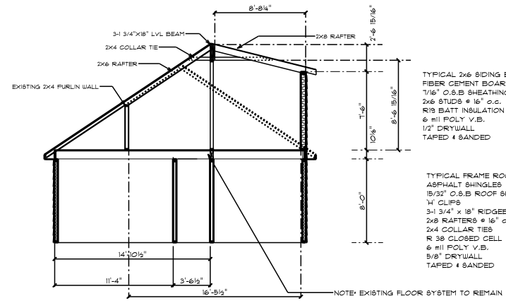
CROSS SECTION SCALE: 1/4" = 1'-0"
