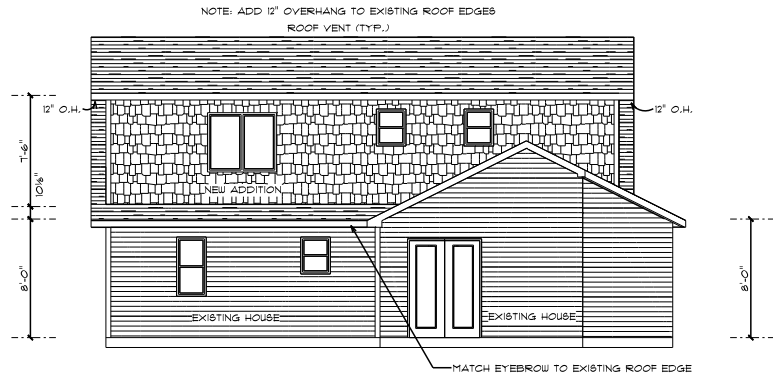
REAR ELEVATION SCALE: 1/4" = 1'-0"
